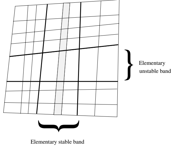
Figure 3: Bands and elementary bands. Nearly vertical lines are leaves of \tilde{\mathcal{G}}^s(\tilde{T}) , and nearly horizontal lines are leaves of \tilde{\mathcal{G}}^u(\tilde{T}) . Thicker lines are periodic leaves. The shaded region is a band which is not an elementary band.
