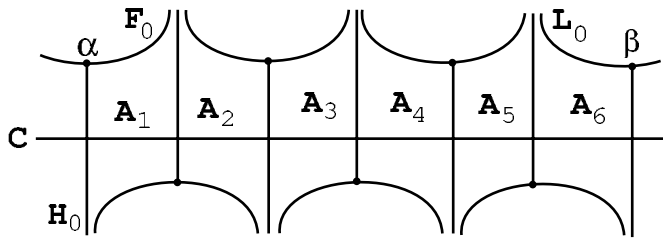
Figure 2: A partial view of a scalloped region. Here C, F_0, L_0 are stable leaves, so this is a s -scalloped region.
