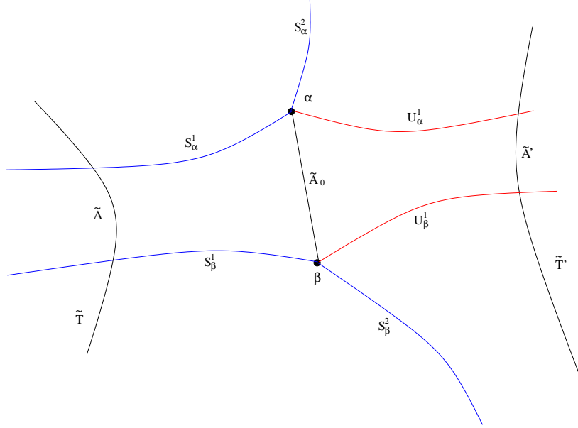
Figure 4: Isolating \tilde{T}' and \tilde{A}_0 by stable prongs.
