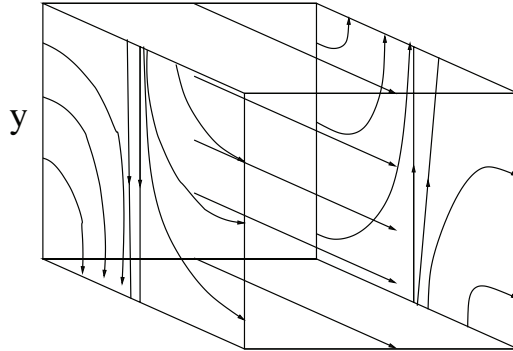
Figure 6: Standard neighborhood of a Birkhoff annulus.
