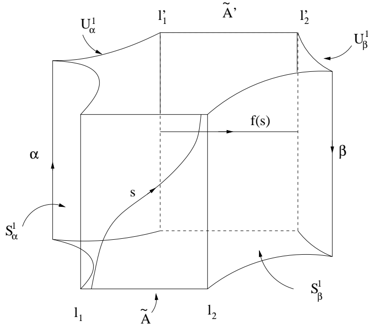
Figure 5: Pushing along the flow a stable leaf in an elementary band.
