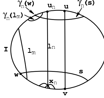
Figure 17: The case of line leaves converging to a limit.
