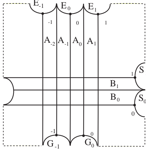
Figure 3: A scalloped region \mathcal{S} . The collections \{E_i\}_{i \in \mathbf{Z}} , \{G_i\}_{i \in \mathbf{Z}} of stable leaves are part of the boundary of \mathcal{S} . In addition \{S_i\}_{i \in \mathbf{Z}} are unstable leaves in the boundary of \mathcal{S} . For better viewing we indent a few of the non separated leaves in (say) \{E_i\}_{i \in \mathbf{Z}} into the square. Similarly for \{G_i\} , \{S_i\} .
