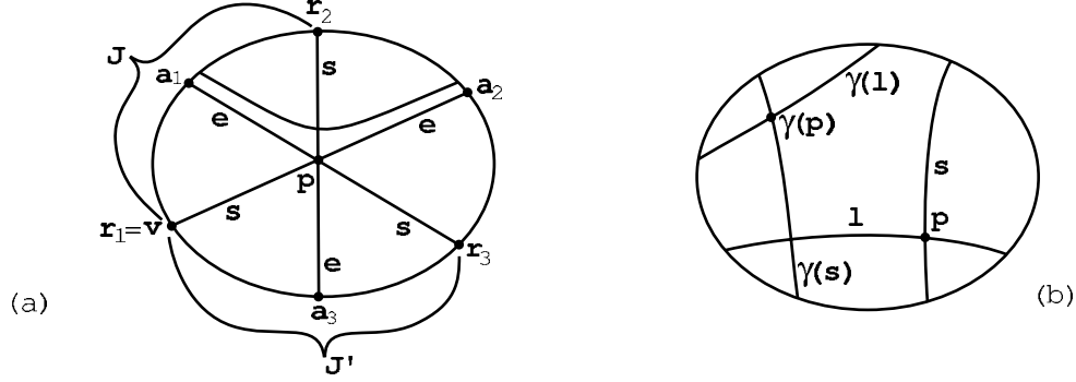
Figure 20: a. Trapping the orbits in the singular case ( n = 3 ), b. An interesting counterexample.
