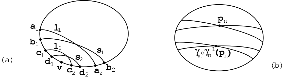
Figure 19: a. Set up in \mathcal{O} , b. Producing fixed points.
