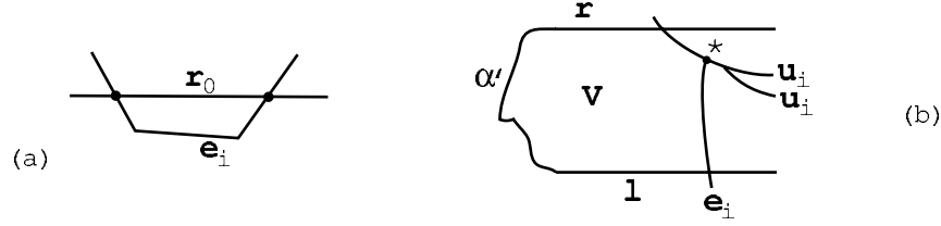
Figure 5: a. Convexity implies connected intersection of r and B_i . b. All rays of u_i stay in V forever. There is a non convex vertex at * .
