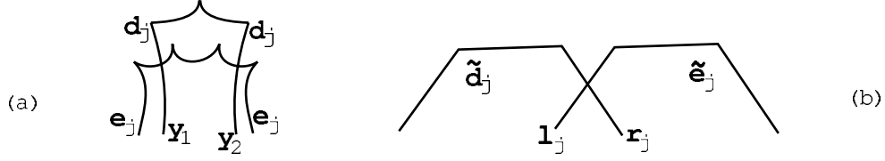
Figure 7: a. The intersection of convex neighborhoods, b. Intersecting master sequences.
