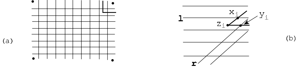
Figure 4: Ideal points for product \mathbf{R} -covered Anosov flow, the dots represent the 4 special points, b. The picture in skewed case.
