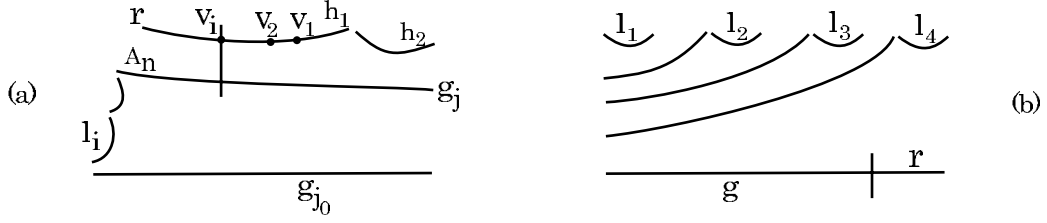
Figure 12: a. Forcing convergence on one side, b. The case that all g_j are equal.
