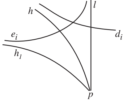
Figure 8: The process of creating standard sequences for rays of \mathcal{O}^s, \mathcal{O}^u . Here the sequence (d_i) of \mathcal{O}^u does not escape compact sets and limits to h leaf of \mathcal{O}^u making a perfect fit with l . There is also the sequence (e_i) of leaves of \mathcal{O}^s whose intersection with h escapes in h and (e_i) limits to a leaf h_1 of \mathcal{O}^s making a perfect fit with h . The leaves l, h_1 are not separated from each other in the leaf space of \mathcal{O}^s .
