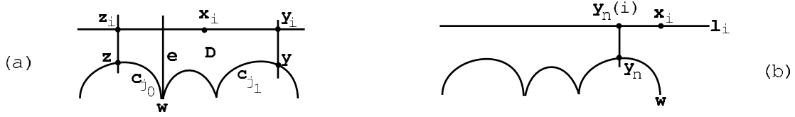
Figure 14: a. The case that x_i is between some unstable leaves, b. The case x_i escapes to one side.
