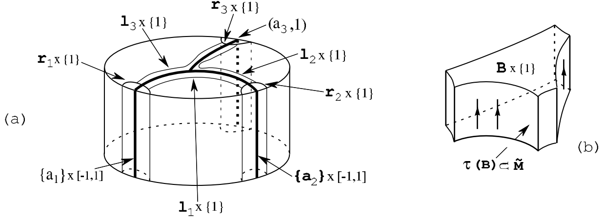
Figure 22: a. The neighborhoods of certain points, b. Flow forward of sections.
