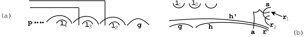
Figure 13: a. The l_i flip to the other side of a leaf non separated from g , b. Convex neighborhood disjoint from all.
