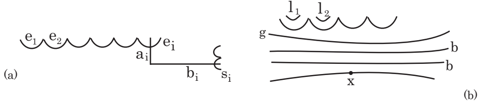
Figure 11: a. Infinitely many non separated leaves converge to a single ideal point, b. A more interesting situation.
