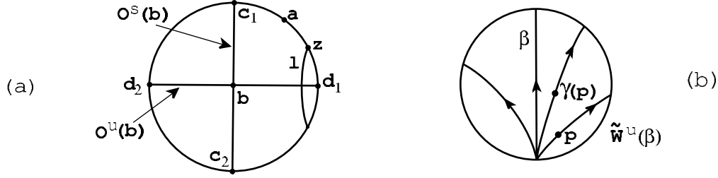
Figure 16: a. The action of \gamma in \mathcal{D} and \partial\mathcal{O} , b. Action of \gamma in \widetilde{W}^u(\beta) .
