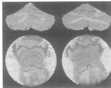
Figure 2. Cerebellar surfaces with PET activation data and fissure labels.
