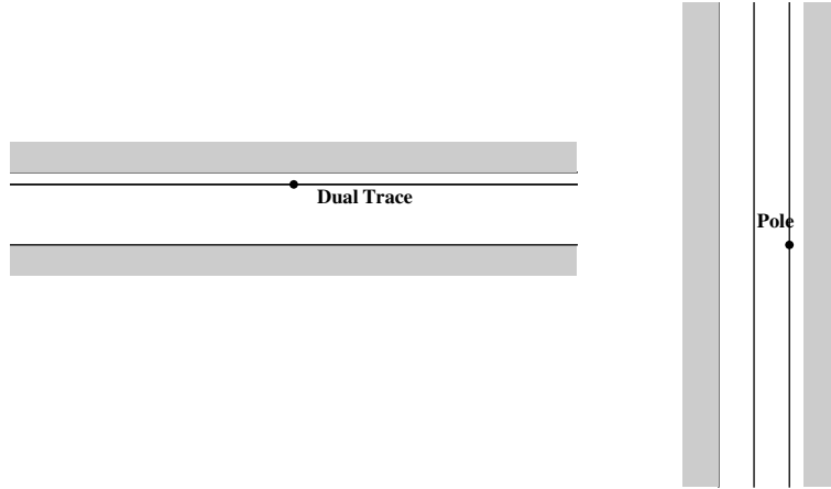
FIGURE 1. The KMS strip and the critical strip
