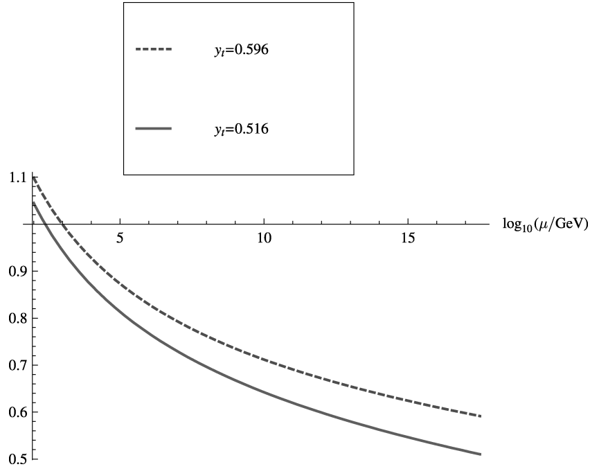
FIGURE 34. The running of the top quark Yukawa coupling.
