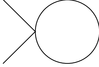
FIGURE 11. Self-energy graph in \phi^4
