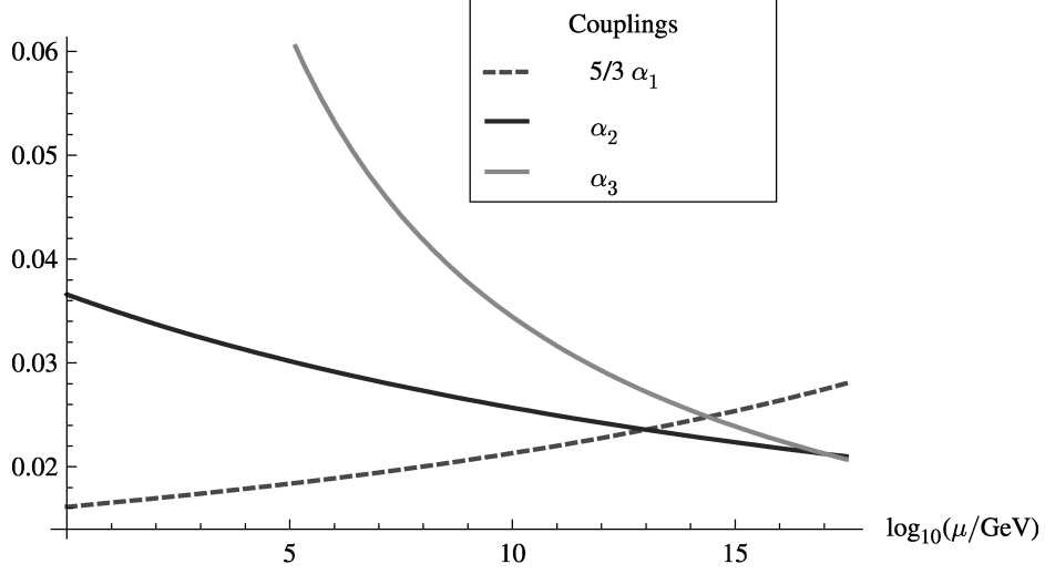
FIGURE 33. The running of the three couplings.
