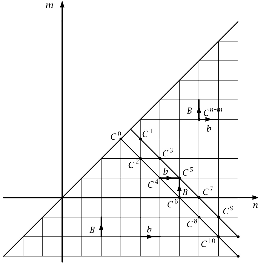
FIGURE 30. The (b, B) bicomplex
