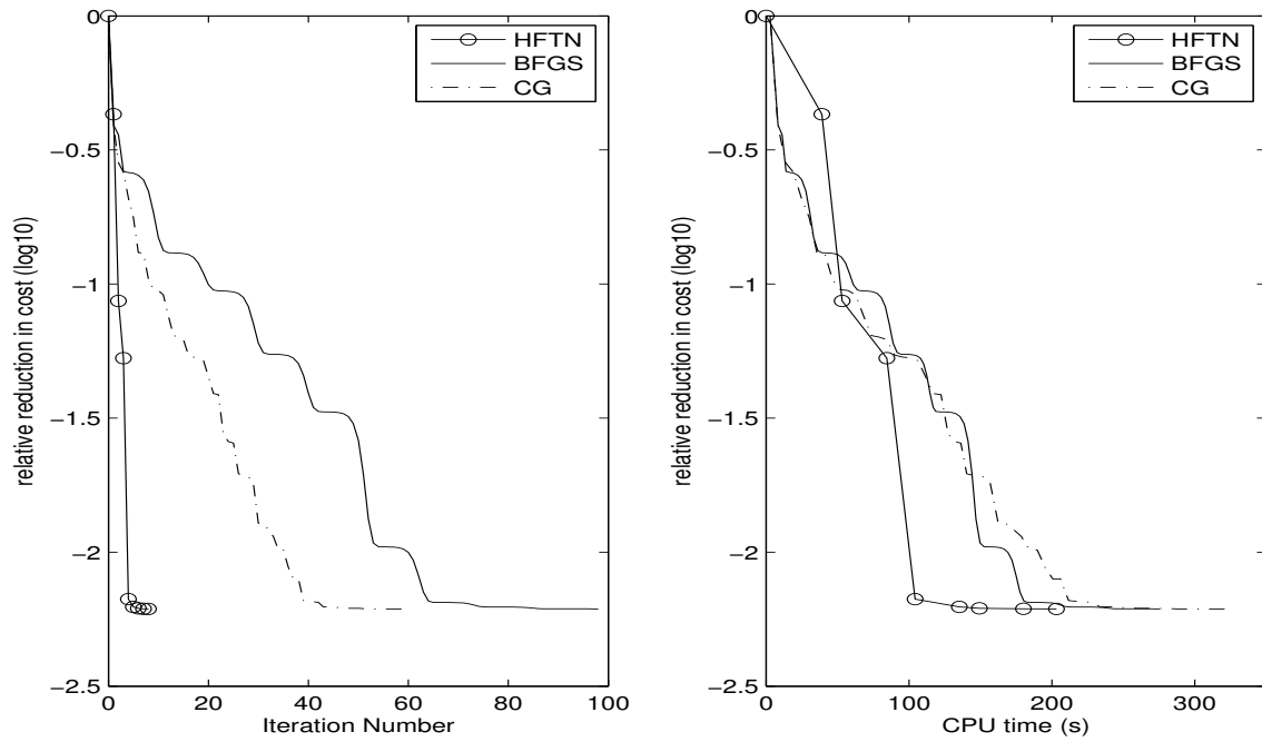
Figure 5. Same as Fig. 4, for the data assimilation experiments in case 1.2.
