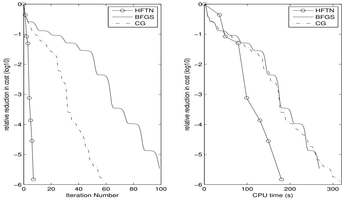
Figure 4. Case 1.1: numerical performance of the optimization algorithms in terms of number of iterations (left figure) and of CPU time (right figure) versus relative reduction in cost functional.
