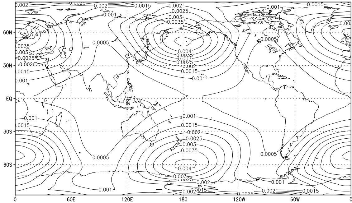
Figure 6. Isopleths of the errors in the retrieved initial conditions measured in the total energy norm.
