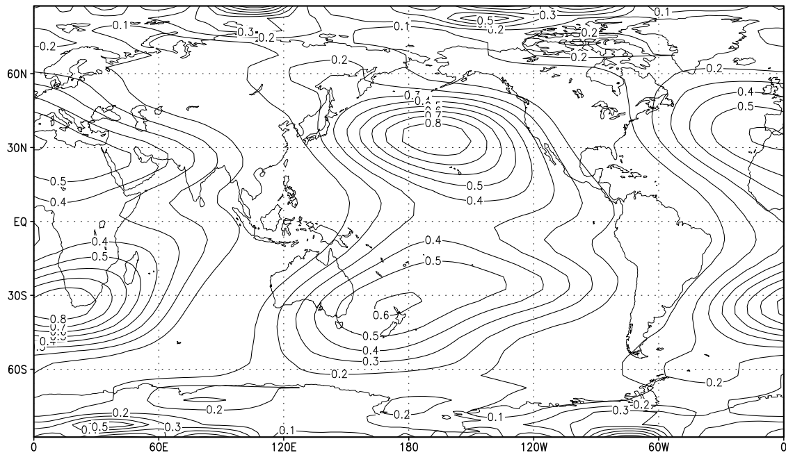
Figure 9. Isopleths of the errors in the retrieved initial conditions measured in the total energy norm.
