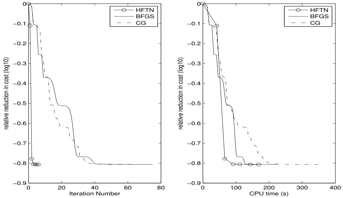
Figure 7. Same as Fig. 4, for the data assimilation experiments in case 2.1.
