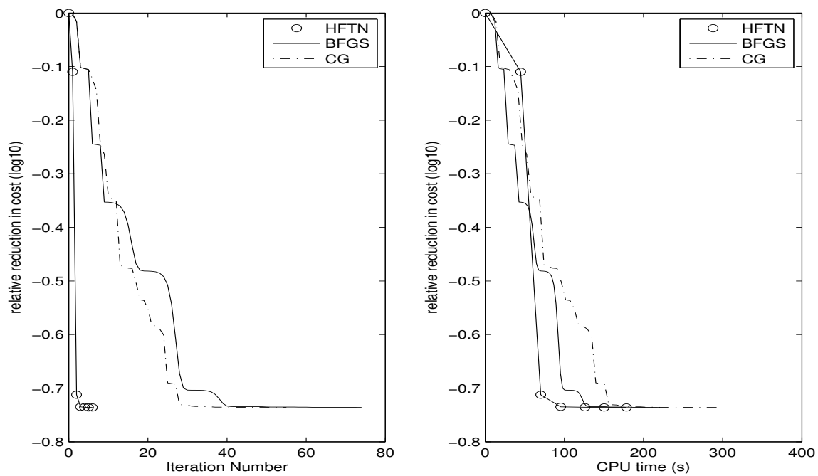
Figure 8. Same as Fig. 4, for the data assimilation experiments in case 2.2.
