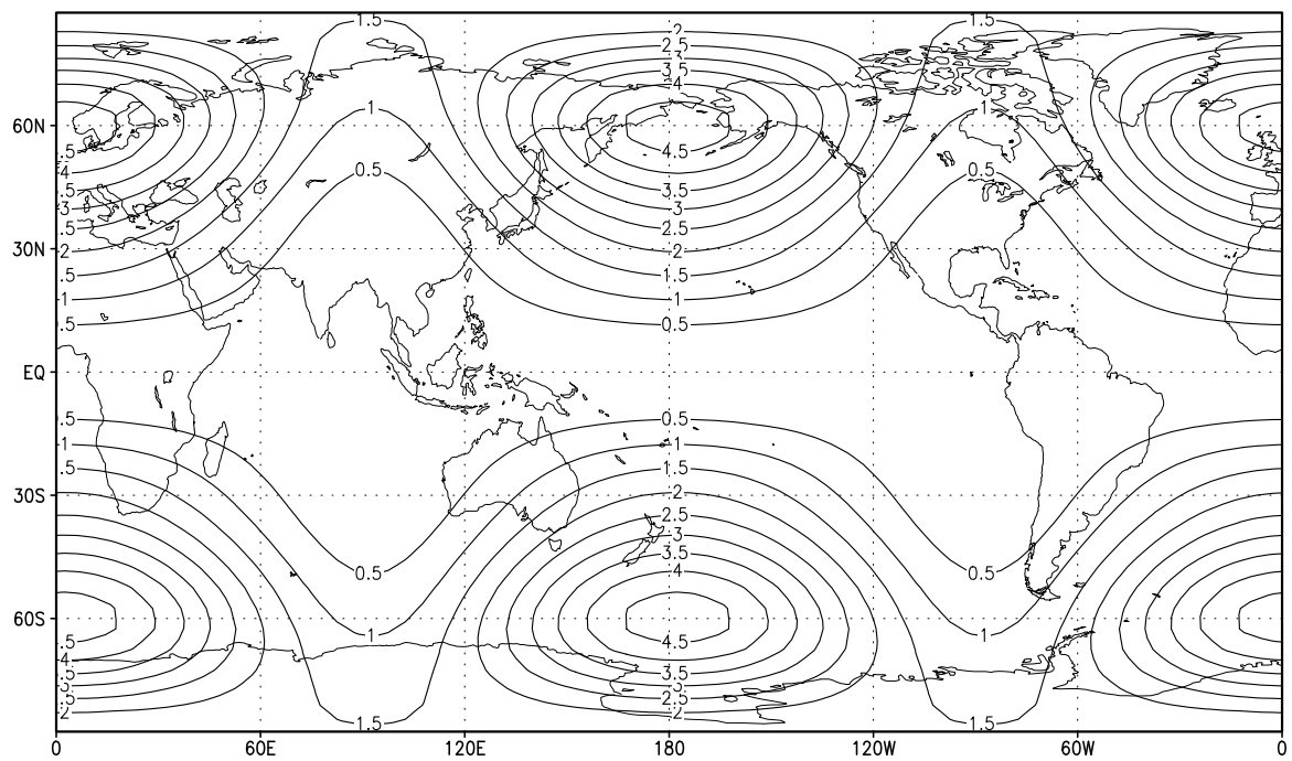
Figure 2. Isopleths of the errors in the first guess (background) estimate to initial conditions. At each grid point the magnitude of the error is evaluated in the total energy norm.
