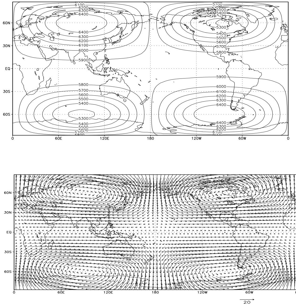
Figure 1. Configuration of the reference initial state of the 2D global shallow water model. Top figure: isopleths of the geopotential height field h in meters. Bottom figure: the velocity vector field (u, v) .
