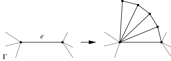
FIGURE 9. Adding a lemon to a graph.
