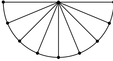
FIGURE 5. The 8th lemon graph \Lambda_8 .
