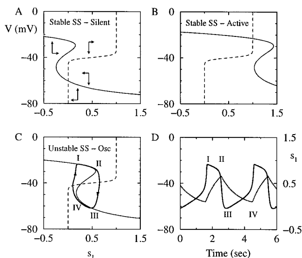
FIGURE 6 Phase plane analysis of fast bursting. The system is reduced to two variables by setting n = n_{\infty}(V) and fixing s_2 at 1.0 (A), -1.0 (B), and 0.346 (C and D). Parameters are as in Fig. 2 except the slope factor for the Boltzmann function s_{1\infty}(V) in Eq. 9 is 1, and g_{s1} = 50 pS. In A-C, light solid curves are V nullclines, dashed curves are s_1 nullclines. Heavy solid curve is the V - s_1 trajectory in C and V time course in D. Dotted line in D is the s_1 time course. SS, steady state. See text for details.
