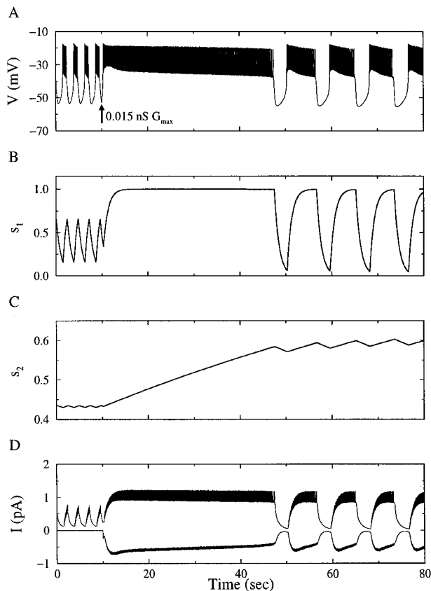
FIGURE 8 Simulated dynamic clamp protocol. Artificial inward current (Eqs. 12–14) with G_{\max} = 0.015 nS and K = 2.0 s ^{-1} added to model equations at t = 10 s. In D , I_{s1} is the current with upward deflections and I_{\text{Clamp}} the current with downward deflections.
