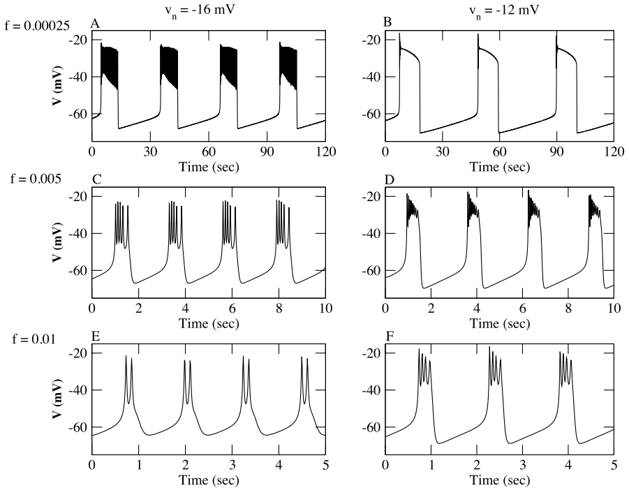
Fig. 5 Bursting oscillations generated with the Chay–Keizer model and different values of f and v_n . For the left panels v_n = -16 mV, and for the right panels v_n = -12 mV. (A), (B) f = 0.00025 . (C), (D) f = 0.005 . (E), (F) f = 0.01
