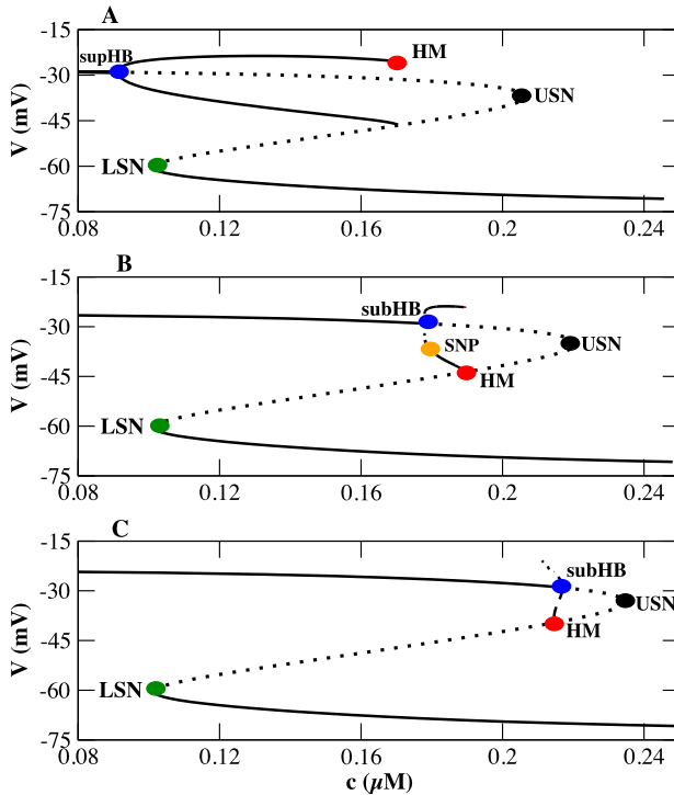
Fig. 4 Effects of shifting the n_\infty(V) curve rightward. (A) The bifurcation structure for plateau bursting using default values (Table 1). (B) A transitional bifurcation structure obtained by increasing v_n to -14 mV. (C) The bifurcation structure for pseudo-plateau bursting obtained with v_n = -12 mV
