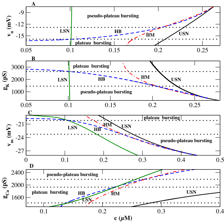
Fig. 6 (Color online) Two-parameter bifurcation diagrams illustrating regions of plateau and pseudo-plateau bursting. The green (LSN), blue (HB), red (HM), and black (USN) curves represent the lower saddle node, Hopf, homoclinic, and upper saddle node bifurcation points, respectively. (A), (C) The midpoints of activation curves are varied. (B), (D) Current conductances are varied. In panel D, the region below the bottom dotted curve is neither plateau nor pseudo-plateau bursting since the order is c_{LSN} < c_{HB} < c_{HM} < c_{USN}
