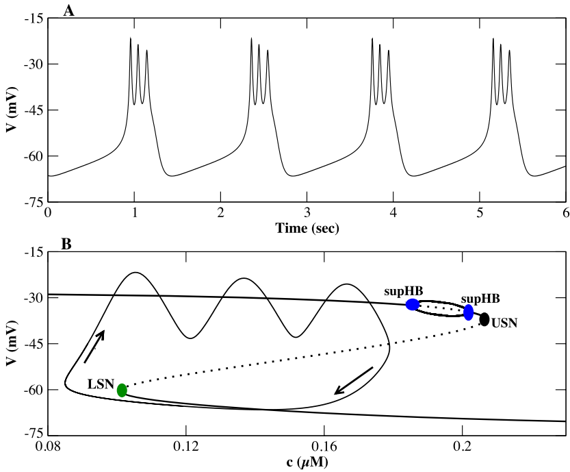
Fig. 2 Pseudo-plateau bursting generated with the Chay–Keizer model by increasing the speed of \text{K}^+ current activation. (A) When \tau_n is decreased to 17.1 ms and f is increased to 0.01, pseudo-plateau bursting is produced. (B) The fast-subsystem bifurcation structure, in which the upper branch is stabilized. There are two supercritical Hopf bifurcations connected by a branch of stable periodic solutions, which differs from Fig. 1F
