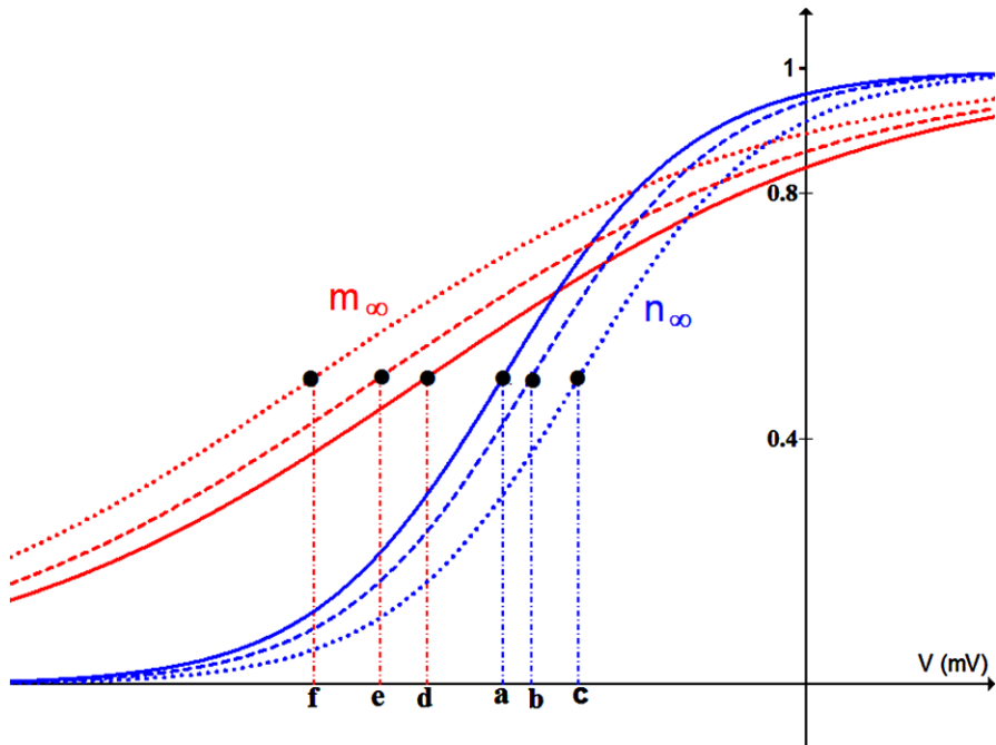
Fig. 3 Steady state functions for the K^+ current activation variable n (the n_\infty(V) curve, blue) and the Ca^{2+} current activation variable m (the m_\infty curve, red). When v_n is increased from -16 mV (point a) to -14.5 mV (point b) or -12 mV (point c), the n_\infty curve shifts to the right. This makes the delayed rectifier channels activate at higher voltages. When v_m is decreased from -20 mV (point d) to -22.5 mV (point e) or -26 mV (point f), the m_\infty curve shifts to the left. This makes the Ca^{2+} channels activate at lower voltages. When the m_\infty and n_\infty curves are sufficiently far apart, pseudo-plateau bursting is produced
