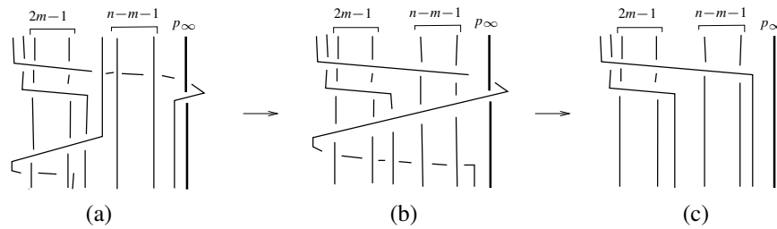
Figure 18: General case
