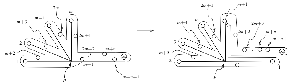
Figure 23: Exchanging the roles of q and p_\infty for \mathfrak{g}'_{m,n} : \infty in the figure indicates p_\infty
