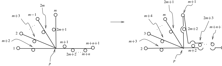
Figure 19: Graph map h_{m,n} for \phi_{\sigma_{m,n}}
