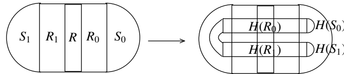
Figure 26: Smale-horseshoe map
