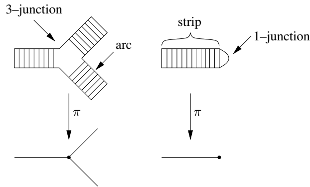
Figure 7: Fibred surface
