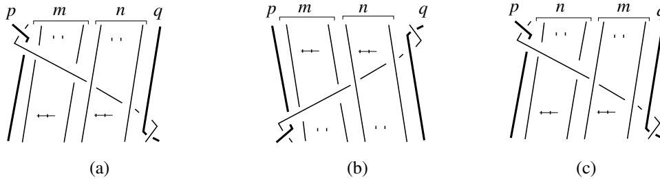
Figure 9: Symmetry of \beta_{m,n}^+
