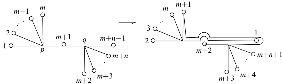
Figure 12: Graph map \mathfrak{g}_{m,n} for \phi_{\beta_{m,n}}
