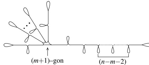
Figure 21: Train track \tau_{h,m,n}
