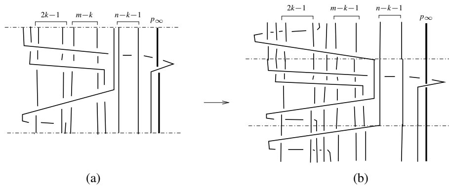
Figure 15: Induction step
