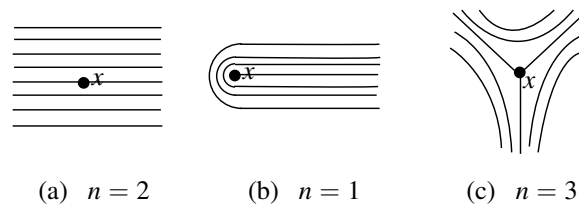
Figure 4: Local picture of a singular foliation
