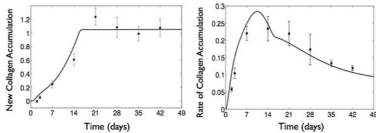
Fig. 8 Comparison of model simulations and experimental data during normal wound healing. Data from Madden and Peacock (1971). WS_0 = 0.6 with pathogen, inflammation and fibroblast all initially zero. In the left panel, data were scaled as described in the text so that they represented the same quantity as COL . In the right panel they were scaled to represent the same quantity as the production term from Eq. (12)
