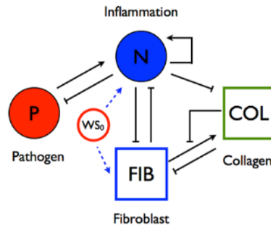
Fig. 1 Model schematic for collagen accumulation model where WS_0 is the initial wound size. The creation of a wound triggers the recruitment of fibroblast from the healthy tissue at the edge of the wound as well as the inflammatory response, dashed arrows . The fibroblasts proliferate and migrate. Arrows represent up regulation, while bars represent down regulation and/or inhibition
