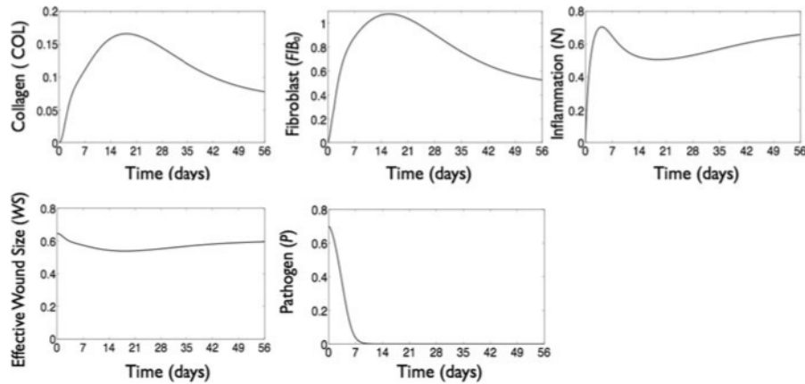
Fig. 11 Wound healing in an infected, oxygen depleted wound. Transients for collagen ( COL ), fibroblast ( FIB_a ), inflammation ( N ), effective wound size ( WS ) and pathogen ( P ) versus days of healing with P_0 = 0.7 , WS_0 = 0.6 , and O_2 = 22 . All other variables were initially set to background levels, COL = 0 , N = 0 , FIB_p = 10 , FIB_m = 0 , and FIB_a = 0
