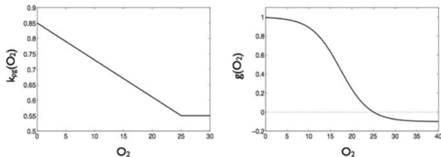
Fig. 4 Auxiliary functions for oxygen. k_{pg}(O_2) and g(O_2) . Plots of the functions used to implement the effects of altering local tissue O_2 above or below O_{crit} = 25
