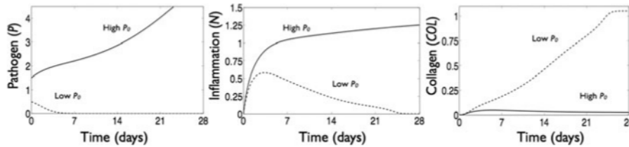
Fig. 9 Transient solutions of wound healing with high and low initial infection levels. Solid line — P_0 = 1.5 and dashed line — P_0 = 0.5 . WS_0 = 0.6 and all other variables were initially set to background levels, COL = 0 , N = 0 , FIB_p = 10 , FIB_m = 0 , and FIB_a = 0
