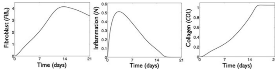
Fig. 5 Transients for normal healing. This wound was created by setting WS_0 = 0.6 with all model variables initially set to background levels, COL = 0 , N = 0 , FIB_p = 10 , FIB_m = 0 , and FIB_a = 0
