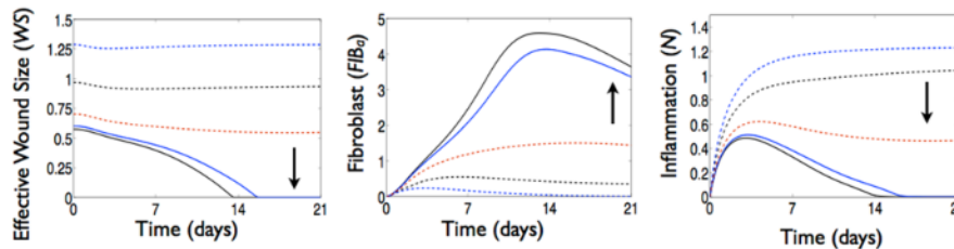
Fig. 10 Wound response to various O_2 levels. All transients have WS_0 = 0.6 and all other variables were initially set to background levels, COL = 0 , N = 0 , FIB_p = 10 , FIB_m = 0 , and FIB_a = 0 . The arrow indicates the direction of increasing O_2 levels (10, 15, 20, 25, 30). Solid curves result in a healed wound. The blue solid curve has O_2 = O_{crit} = 25 and black O_2 = 30 . The dashed curves result in a non-healed wound, red O_2 = 20 , black O_2 = 15 and blue O_2 = 10 (Color figure online)
