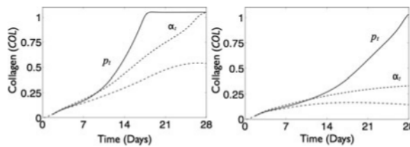
Fig. 12 Collagen accumulation in treated wounds with and without reduced O_2 . Left panel , transients for collagen ( COL ) with normal healing ( dot-dashed ), antibiotic treatment ( dashed , \alpha_t = 10 ), and altered fibroblast ( solid , p_t = 1.3 ) with normal oxygen, P_0 = 0.7 , and WS_0 = 0.6 and all other variables were initially set to background levels, COL = 0 , N = 0 , FIB_p = 10 , FIB_m = 0 , and FIB_a = 0 . Right panel , all parameters and initial conditions are the same as the left panel except O_2 = 20 . All treatments were implemented at t = 2 days
