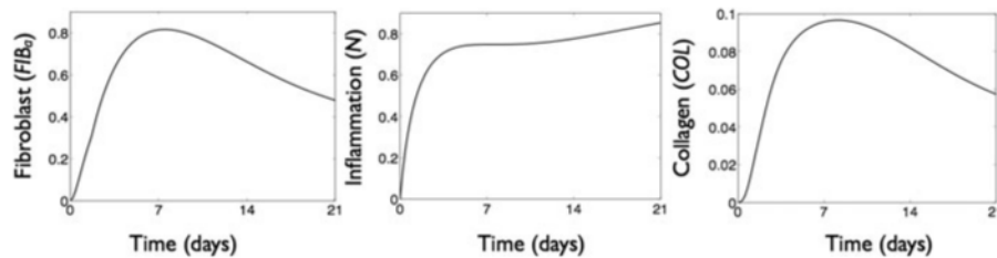
Fig. 6 Transients for a chronic wound. This wound was created by setting WS_0 = 0.8 with all model variables initially set to background levels, COL = 0 , N = 0 , FIB_p = 10 , FIB_m = 0 , and FIB_a = 0
