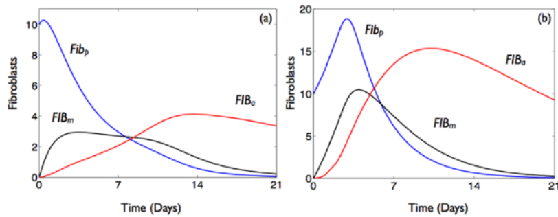
Fig. 2 Fibroblast stages during wound healing with and without an inflammatory response. Transients for proliferating fibroblasts ( FIB_p ), migrating fibroblasts ( FIB_m ) and active fibroblasts ( FIB_a ) with WS_0 = 0.6 . All other variables were initially set to background levels, COL = 0 , N = 0 , FIB_p = 10 , FIB_m = 0 , and FIB_a = 0 . (a) Shows activity with a normal inflammatory response. (b) Shows activity with inflammatory response suppressed
