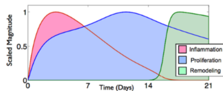
Fig. 7 Stages of wound healing. Transients are plotted for scaled N (red—inflammation), the sum of FIB_m and FIB_a (blue—proliferation) and collagen degradation term from Eq. (12) (green—remodeling). Each transient was scaled by the maximum of the variable model for comparison (Color figure online)
