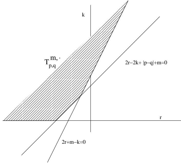
FIGURE 1. The region \Lambda_{p,q} \subset \mathbb{Z}^2 defining \mathcal{T}_{p,q}^{m,*}
