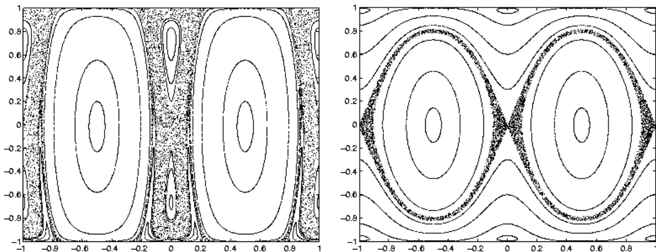
FIG. 2: Phase space structure of the normalized equations (15) with \bar{L} = 2 , \omega = \eta = F = 1 , and \Omega = \epsilon = 0.1 . Left panel: \gamma = 0.8 . Right panel: \gamma = 2 . In both panels the horizontal and vertical axes indicate \bar{g}/\pi and \bar{G}/\bar{L} , respectively.
