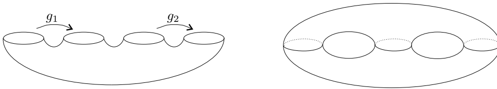
FIGURE 2. A topological side view of the Riemann sphere is shown on the left. The isometric circles of the hyperbolic Möbius transformations g_1 and g_2 , together with their respective images are also shown. The group generated by g_1 and g_2 acts in such a way that a fundamental domain is the exterior of the disks shown on the left. The group simply identifies the isometric circle of g_j with its image, j = 1, 2 , to form the genus 2 Riemann surface shown on the right.
