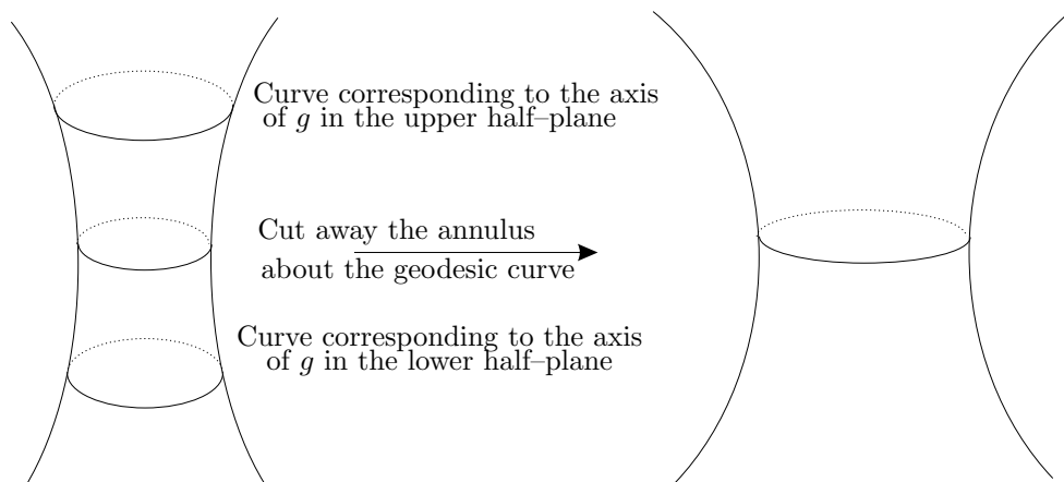
FIGURE 3. The original Schottky uniformized Riemann surface \Gamma/G is deformed by cutting away parts of the handles and identifying the closed curve corresponding to the axis of a hyperbolic Möbius transformation g in the upper half plane with that of the same axis in the lower half-plane. Handles get shorter and thicker as illustrated above.
