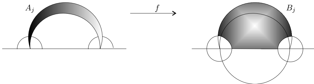
FIGURE 4. The quasiconformal mapping f that makes up the deformation we had to perform on \Gamma/G to get a Fuchsian uniformization stretches the collar on the left to cover the whole shaded collar on the right.
