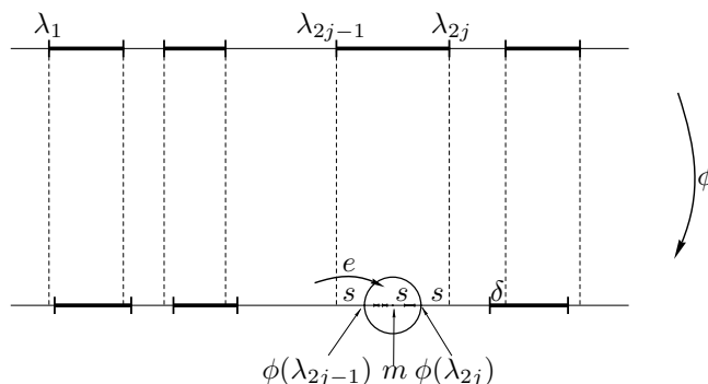
FIGURE 1. The mapping \phi opens a slot of length 4s and replaces it by a disk D of radius s . The higher generation slots are obtained as images of the other slots under an elliptic Möbius transformation e mapping the complement of the closure of disk D onto D itself. Also the other slots move towards the mid-point m of the slot that is being opened. The function \delta measures this movement. The points \phi(\lambda_{2j-1}) and \phi(\lambda_{2j}) are the fixed points of the elliptic transformation e_j corresponding to this opening of a slot.
