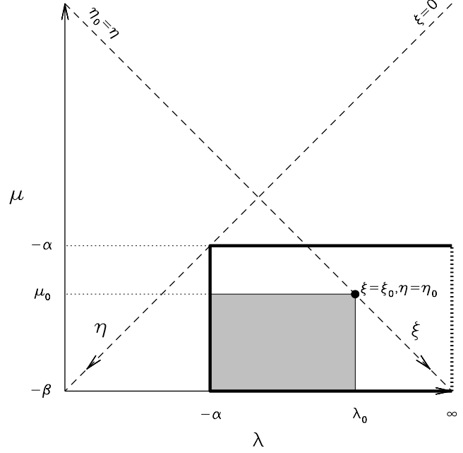
Figure A1. The physically relevant region of the (\lambda, \mu) -plane for the determination of the Riemann–Green function G , overlaid with the new coordinates \xi and \eta (A5). The dot marks the source point of the Riemann–Green function G at (\lambda_0, \mu_0) . This function is non-zero only in the shaded region, which denotes the domain of influence in the (\lambda, \mu) -plane of that source point. Fig. 4 on the other hand shows the (\lambda_0, \mu_0) -plane. It is relevant to the solution for the stress at a single field point (\lambda, \mu) . The hatched region D of Fig. 4 shows the domain of dependence of the field point, that is the portion of the source plane on which the solution at the field point depends.
