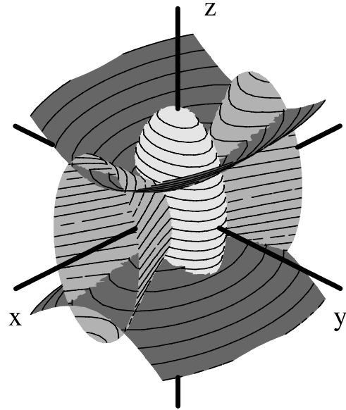
Figure 1. Confocal ellipsoidal coordinates. Surfaces of constant \lambda are ellipsoids, surfaces of constant \mu are hyperboloids of one sheet and surfaces of constant \nu are hyperboloids of two sheets.
