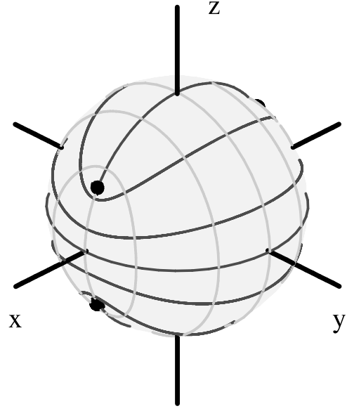
Figure 3. Behaviour of the confocal ellipsoidal coordinates in the limit of large radii r . The surfaces of constant \lambda become spheres. The hyperboloids of constant \mu and \nu approach their asymptotic surfaces, and intersect the sphere on the light and dark curves, respectively. These form an orthogonal curvilinear coordinate system (\mu, \nu) on the sphere. The black dots indicate the transition points ( \mu = \nu = -\beta ) between both sets of curves.
