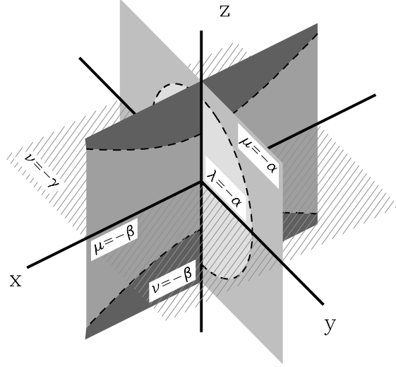
Figure 2. Special surfaces inside ( \lambda = -\alpha ) and outside ( \mu = -\alpha ) the focal ellipse in the plane x = 0 , and inside ( \mu = -\beta ) and outside ( \nu = -\beta ) the two branches of the focal hyperbola in the plane y = 0 and the plane z = 0 ( \nu = -\gamma ).
