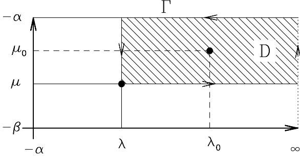
Figure 4. The (\lambda_0, \mu_0) -plane. The total stress at a field point (\lambda, \mu) , consists of the weighted contributions from source points at (\lambda_0, \mu_0) in the domain D , with boundary \Gamma .
