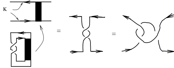
Figure 1: Positive Hopf plumbing
