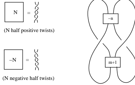
Figure 6: Two bridge link associated to \Gamma_{m,n}
