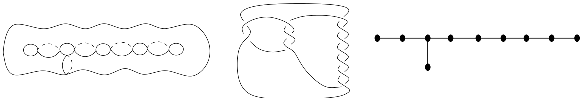
FIGURE 1. Manifestations of Lehmer's number as mapping class, pretzel knot, and Coxeter graph.
