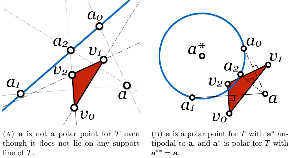
FIGURE 1. Polar points for a given simplex T = [\mathbf{v}_0, \mathbf{v}_1, \mathbf{v}_2] .
