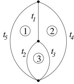
FIGURE 7. Another graph with 3 loops and injective \tau
