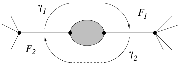
FIGURE 5. Two faces with more than one edge in common.
