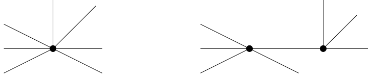
FIGURE 2. A splitting of a graph \Gamma at a vertex v
