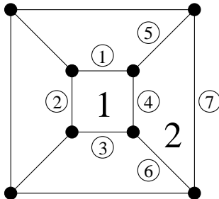
FIGURE 1. An example satisfying Lemma 3.5.
