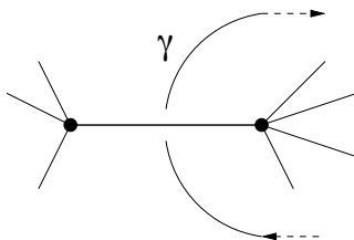
FIGURE 4. An edge not in the boundary of two faces.
