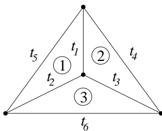
FIGURE 6. The wheel with three spokes graph
