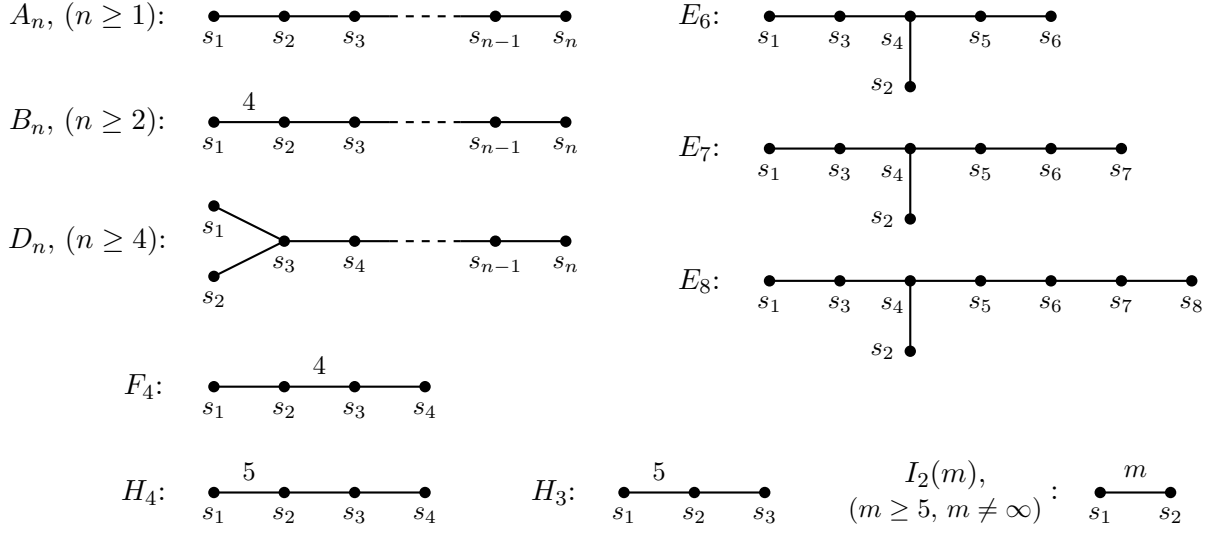
FIGURE 1. Coxeter graphs of irreducible Artin groups of spherical type.
