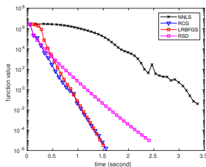
Figure: A representative result with m = n = 50000 , r = 10 , OS = 6
