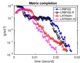
Figure: A representative trajectory
